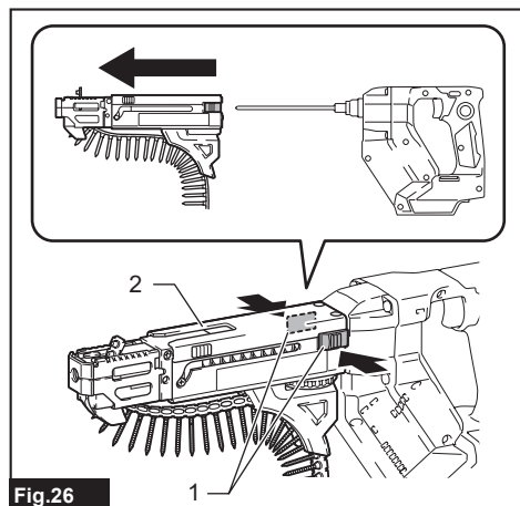
► 1. Release buttons 2. Casing
