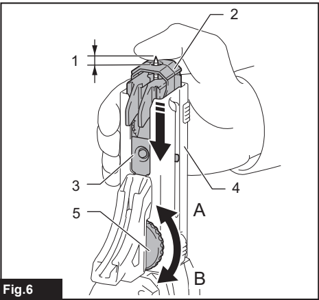
Fig.6 ► 1. Approx. 6 mm (1/4") 2. Stopper base 3. Feeder box 4. Casing 5. Adjusting dial
